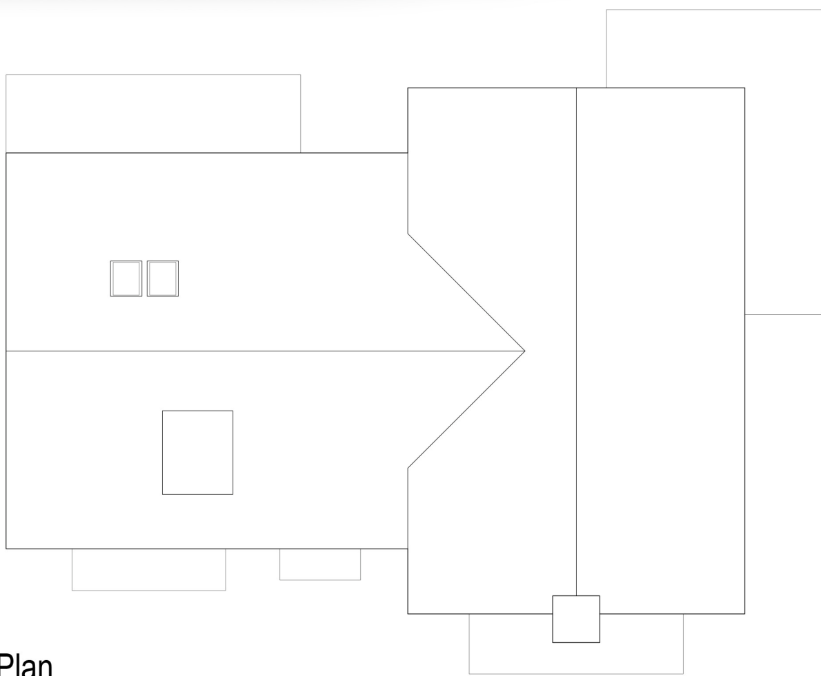
Roof Plan
